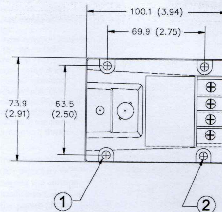
Figure 1: 990 Vibration Transmitter Dimensions (top view)
