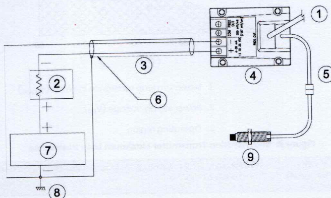
Figure 6: 3300 NSv Extension Cable
